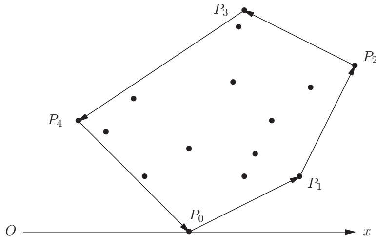
FIG. 8.13 – Enveloppe convexe
