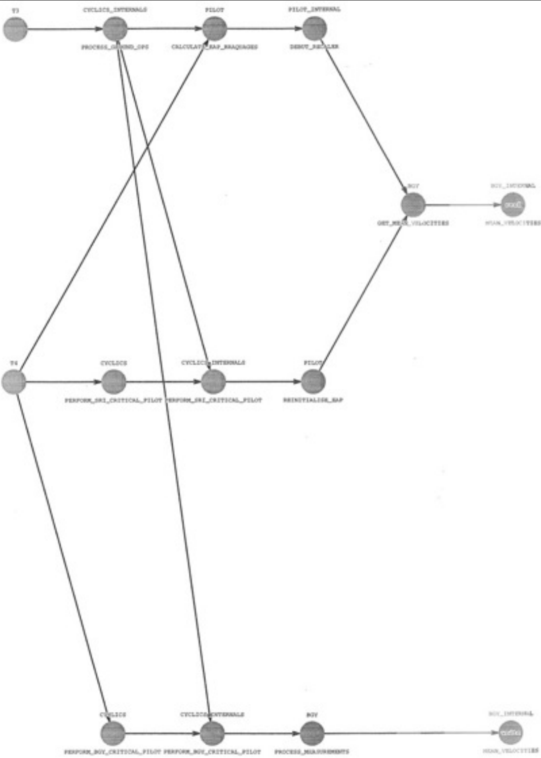
Possibly concurrent accesses for non-scalar #8: BOY INTERNAL.MEAN VELOCITIES
