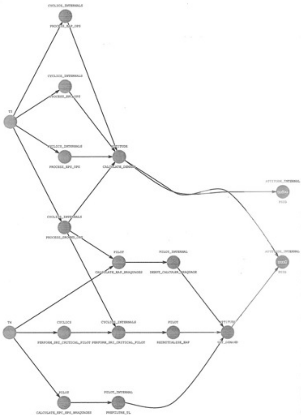
Possibly concurrent accesses for non-scalar #6: ATTITUDE_INTERNAL.PSID
