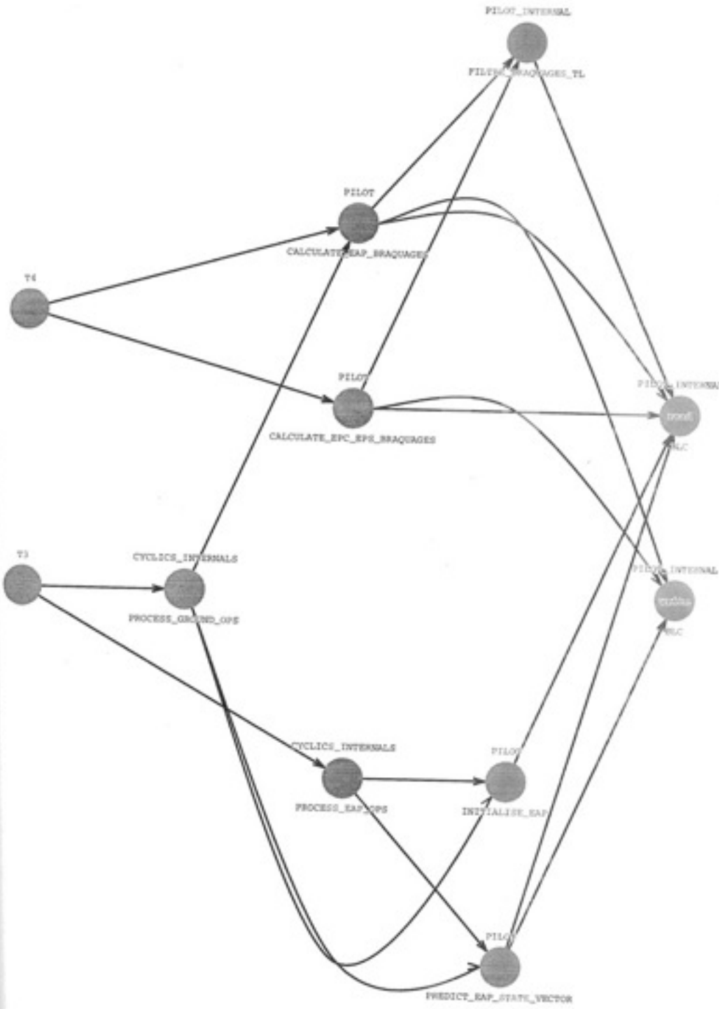
Possibly concurrent accesses for variable $111. (see comments)
