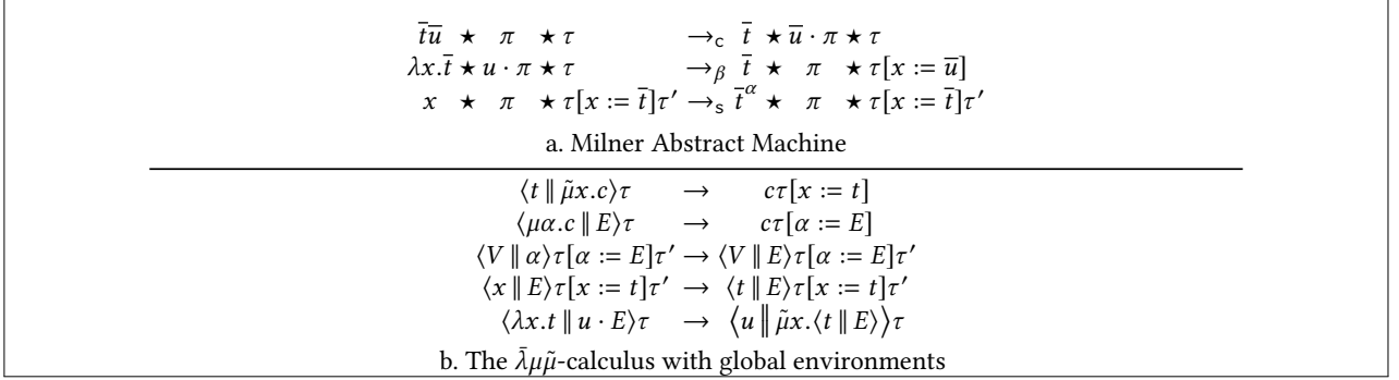
Figure 11. Milner Abstract Machine and \bar{\lambda}\mu\tilde{\mu} -calculus
